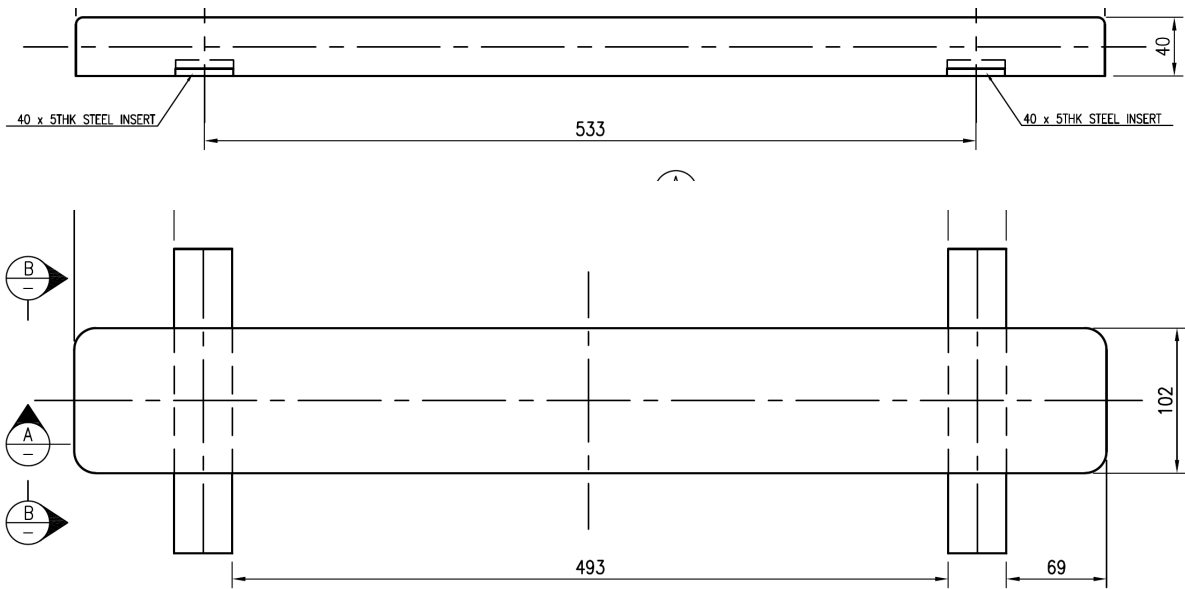
PLAN OF ZGW42 ANODE
