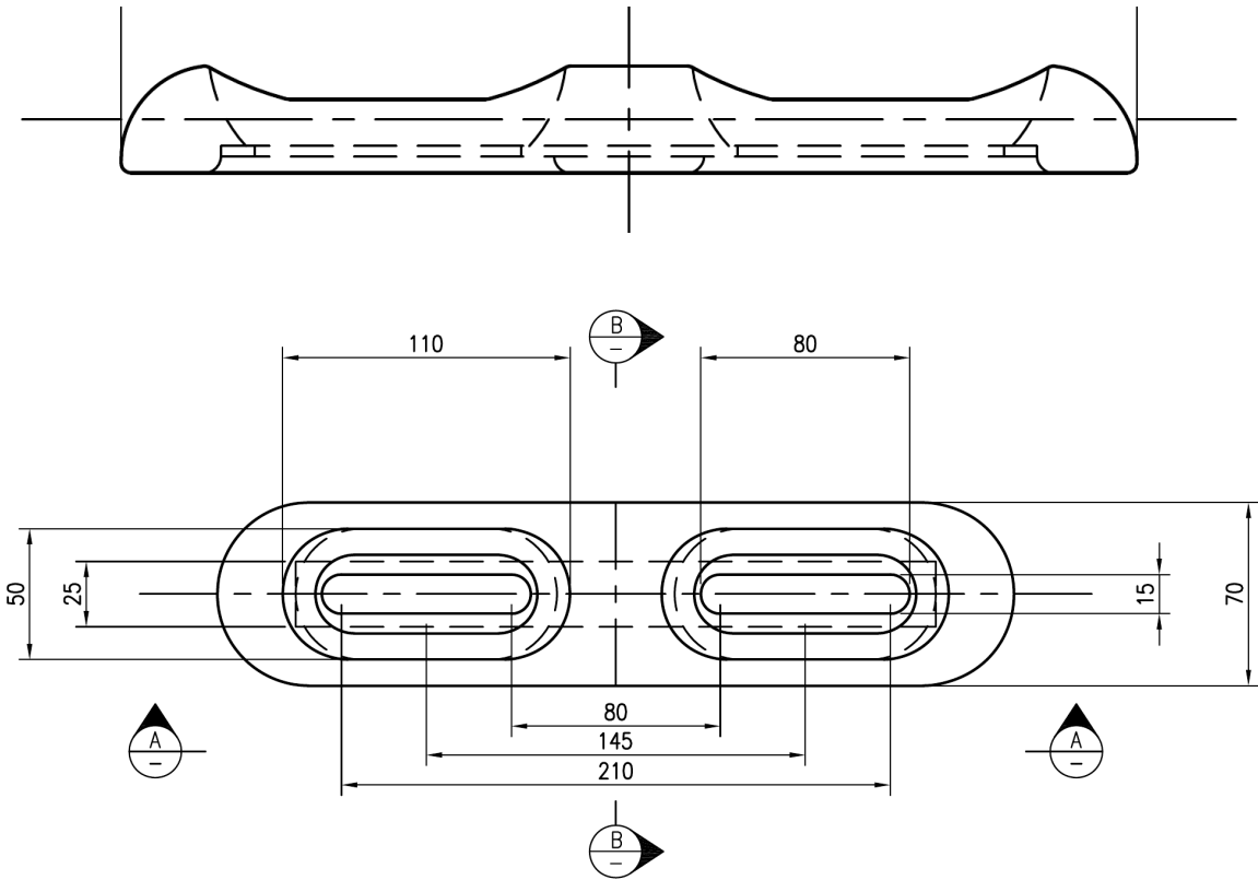
PLAN OF ZGS7C ANODE
