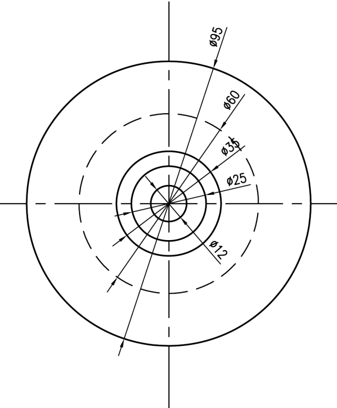
PLAN OF ZGR2 ANODE SCALE 1:1
