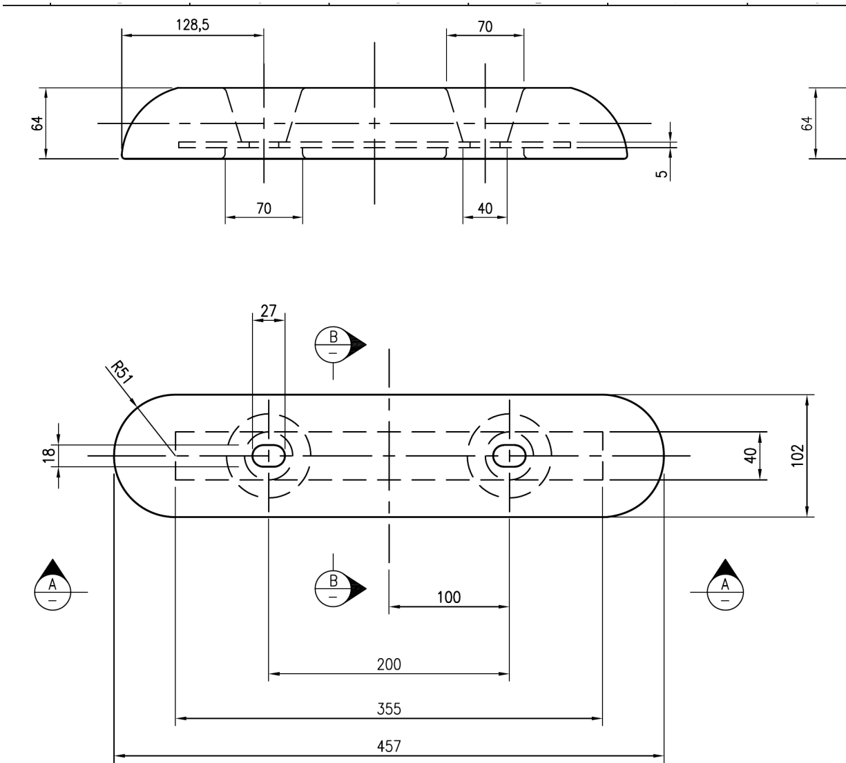
PLAN OF CEGB25R ANODE
