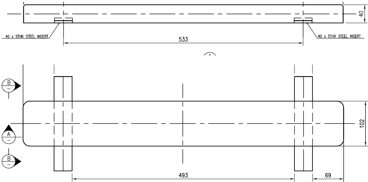
PLAN OF AGW42 ANODE
