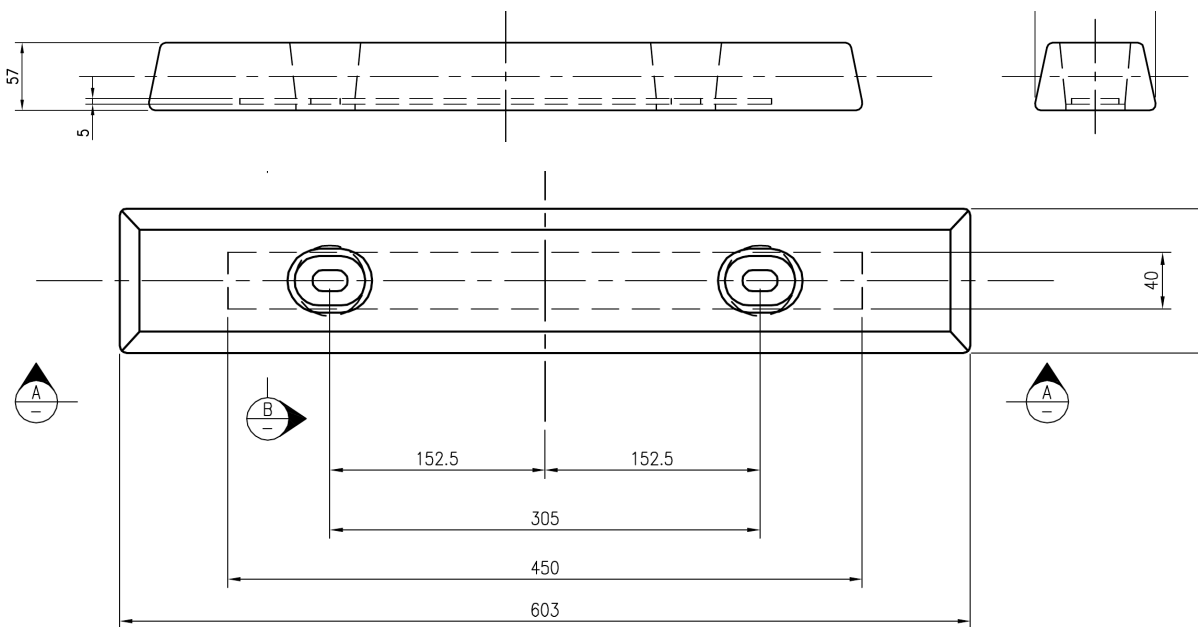
PLAN OF AGS40 ANODE
