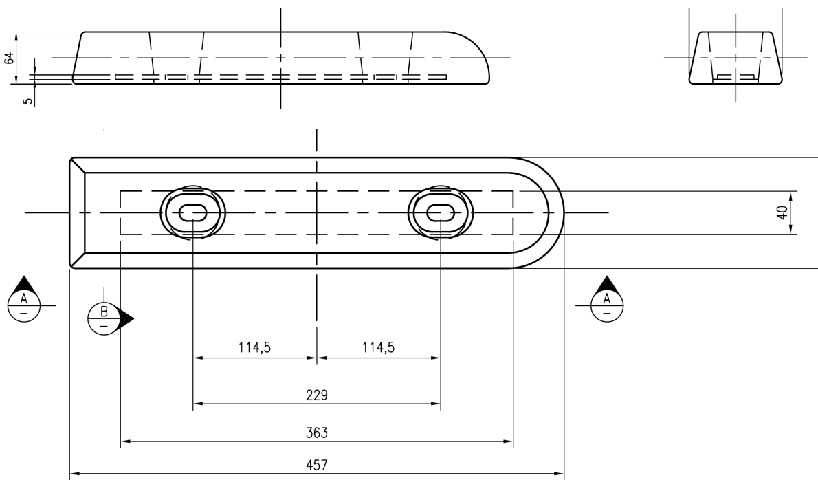
PLAN OF AGS30 ANODE
