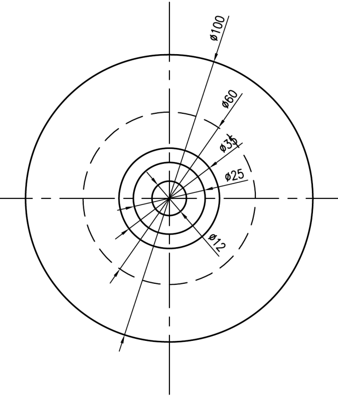
PLAN OF AGR2 ANODE SCALE 1:1
